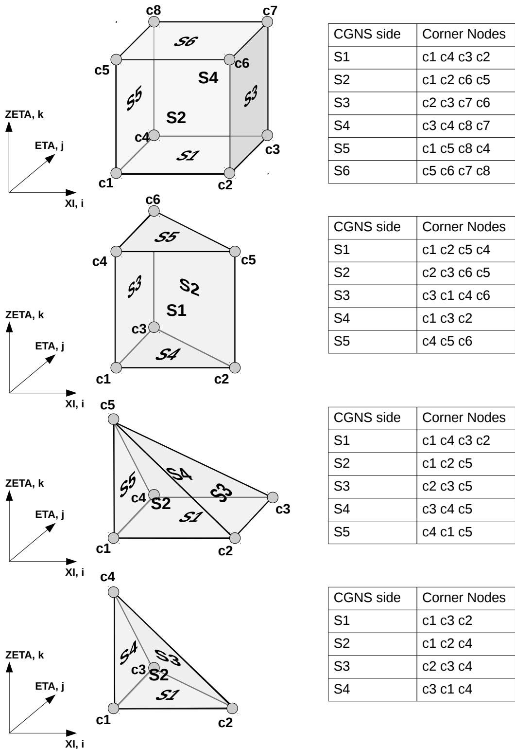
Figure 4.2: Definition of corner nodes, side order and side orientation, from CGNS SIDS.
